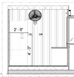
7. WALL ELEVATION C 1 : 50
